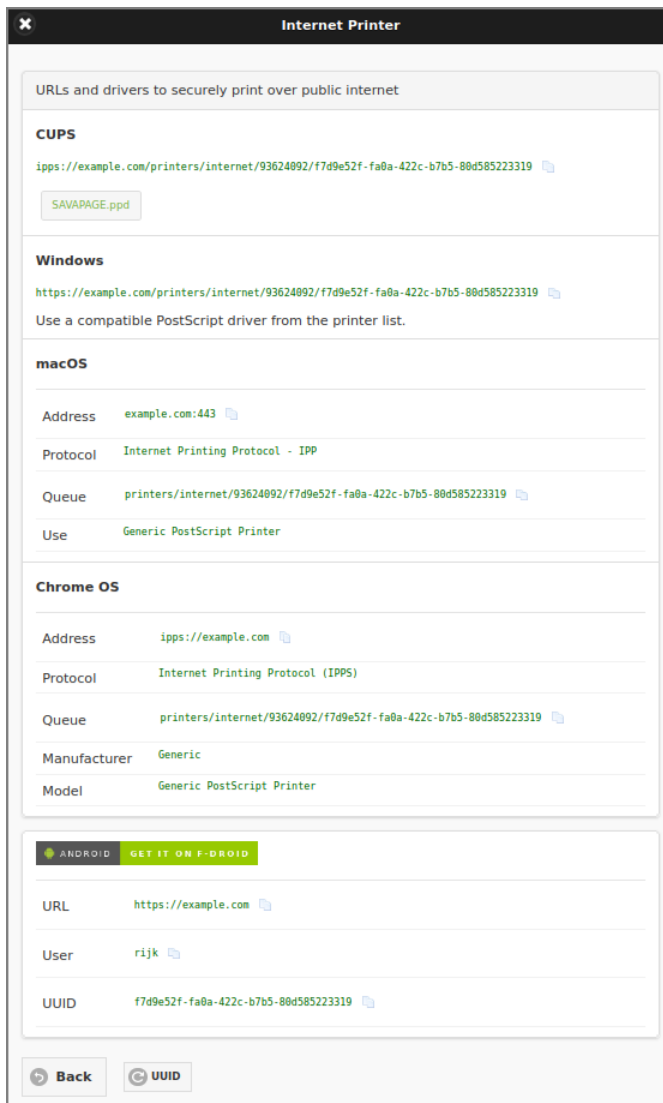
Figure 3.75. User Web App: User Details - Internet Printer
