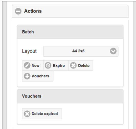
Figure 4.163. Admin Web App: Voucher Actions
