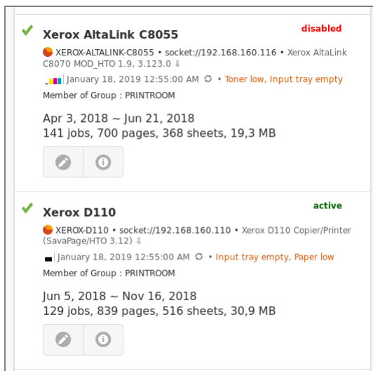
Figure 4.61. Admin Web App: Proxy Printer - List Items
