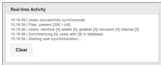
Figure 4.20. Admin Web App: Dashboard - Real-time Activity
