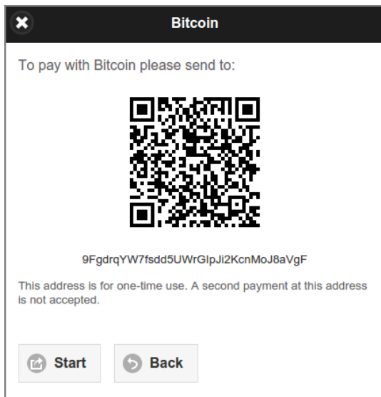
Figure 3.84. User Web App: Send Bitcoins
