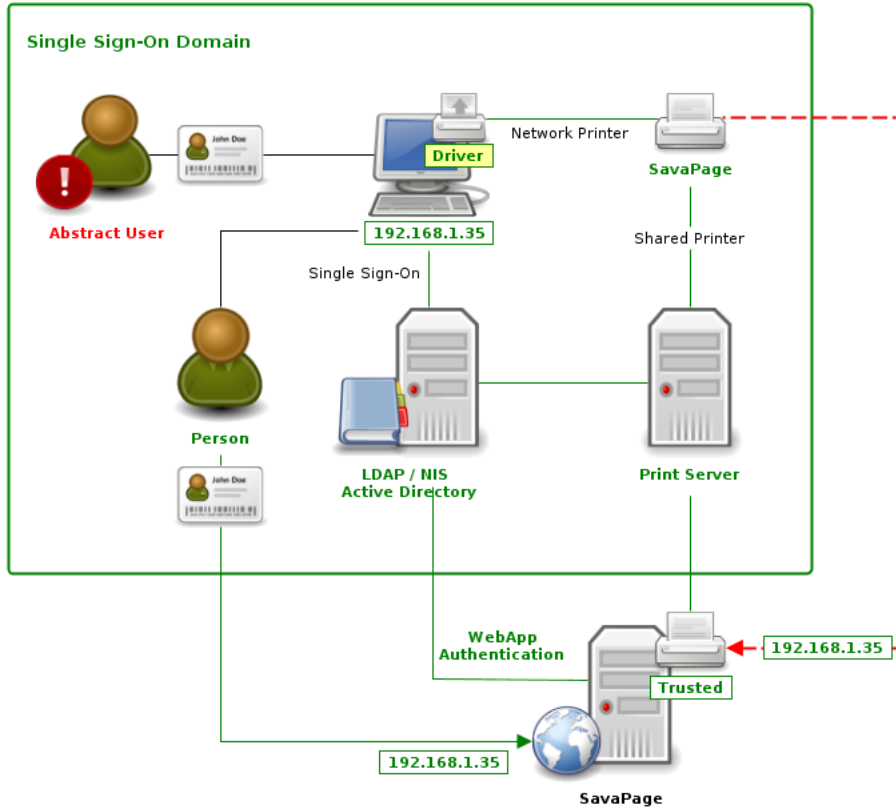
Figure 15.2. IP Based Authentication for Abstract User
