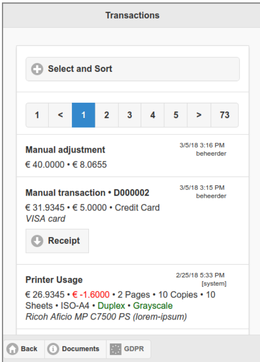
Figure 3.65. User Web App: Log - Transactions
