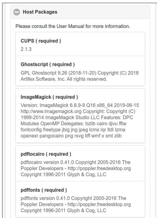
Figure 4.158. Admin Web App: About - Host Packages - 1/3
